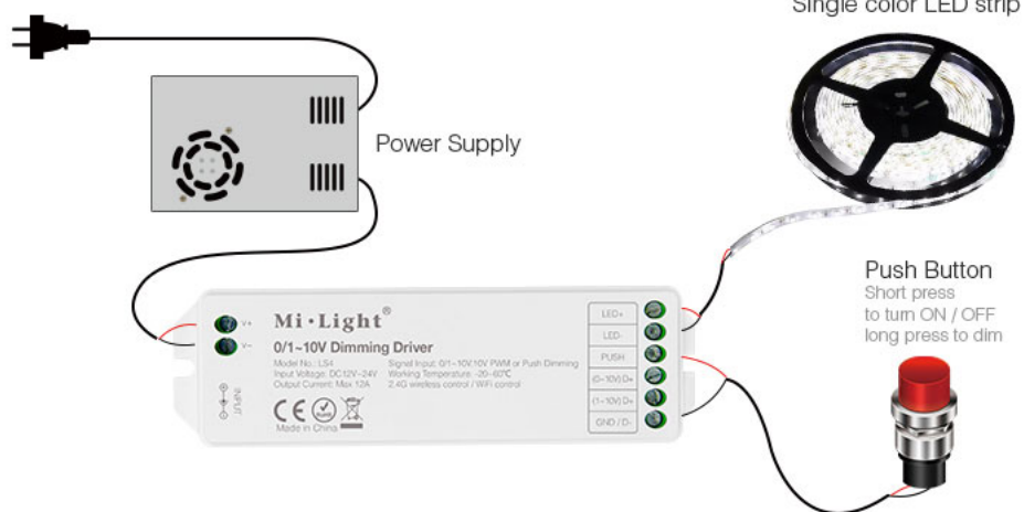
Push button connection diagram
