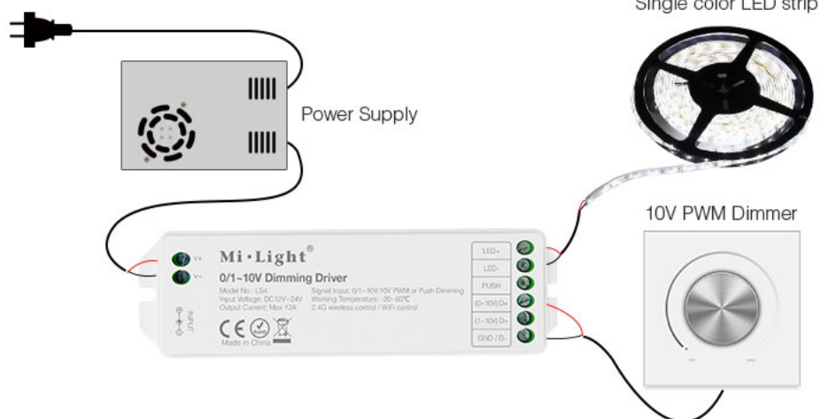
10V PWM dimming panel connection diagram
