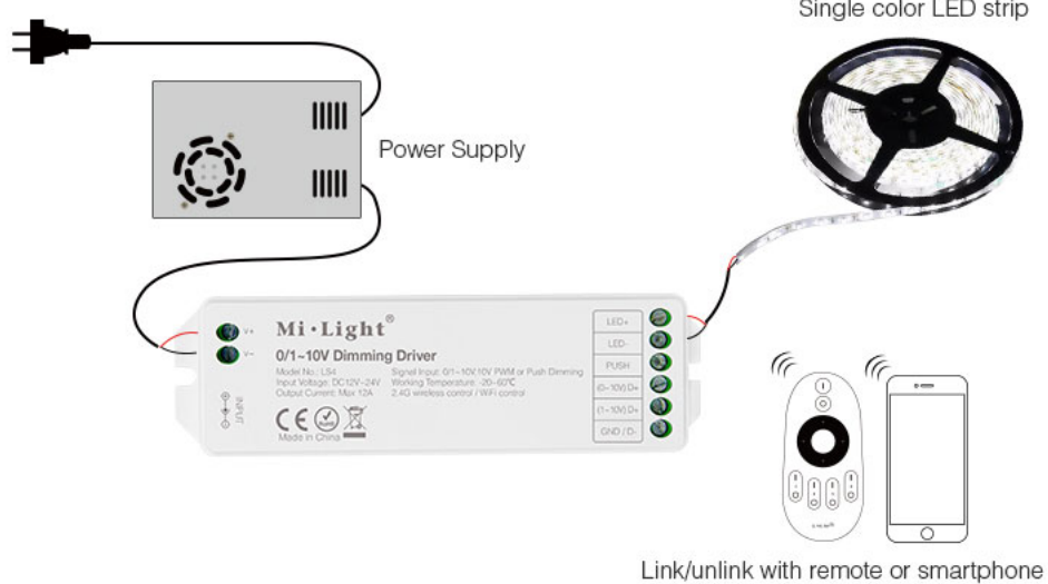
Wireless remote control connection diagram
