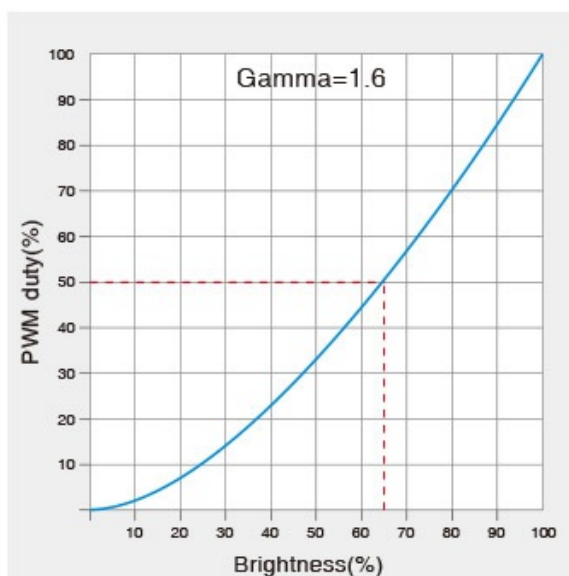
Logarithmic dimming
